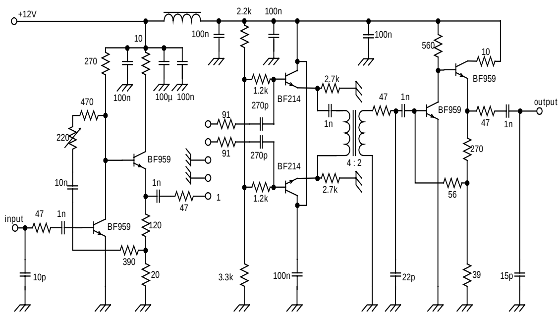
Fig.2 Evaluation circuit
