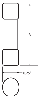
Dimensional Data
