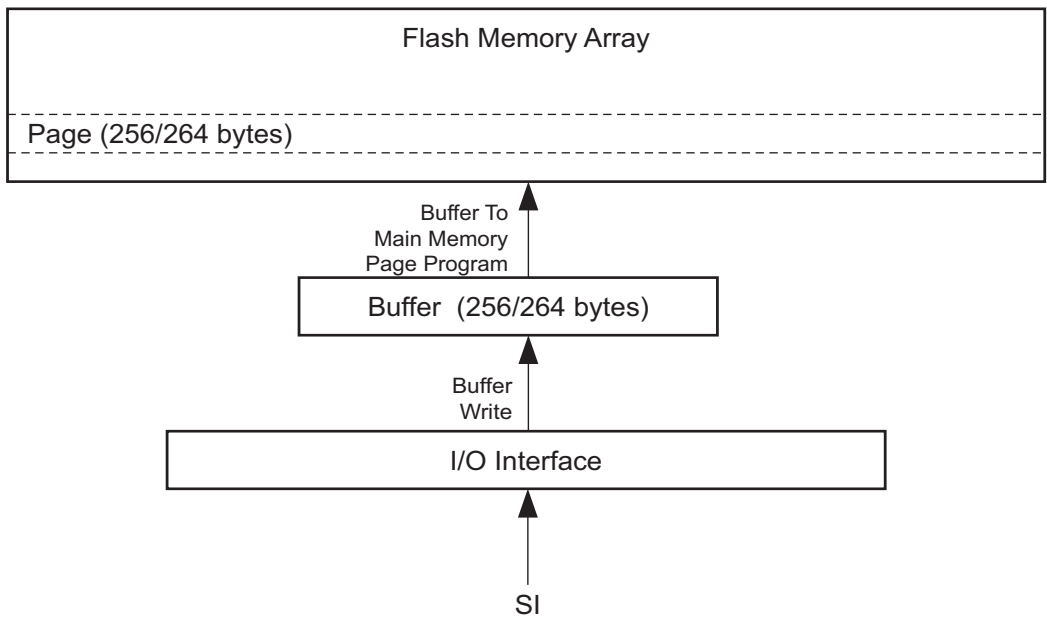
Figure 23-1. Block Diagram
