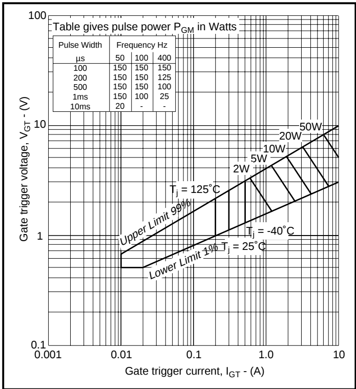
Fig.5 Gate characteristics
