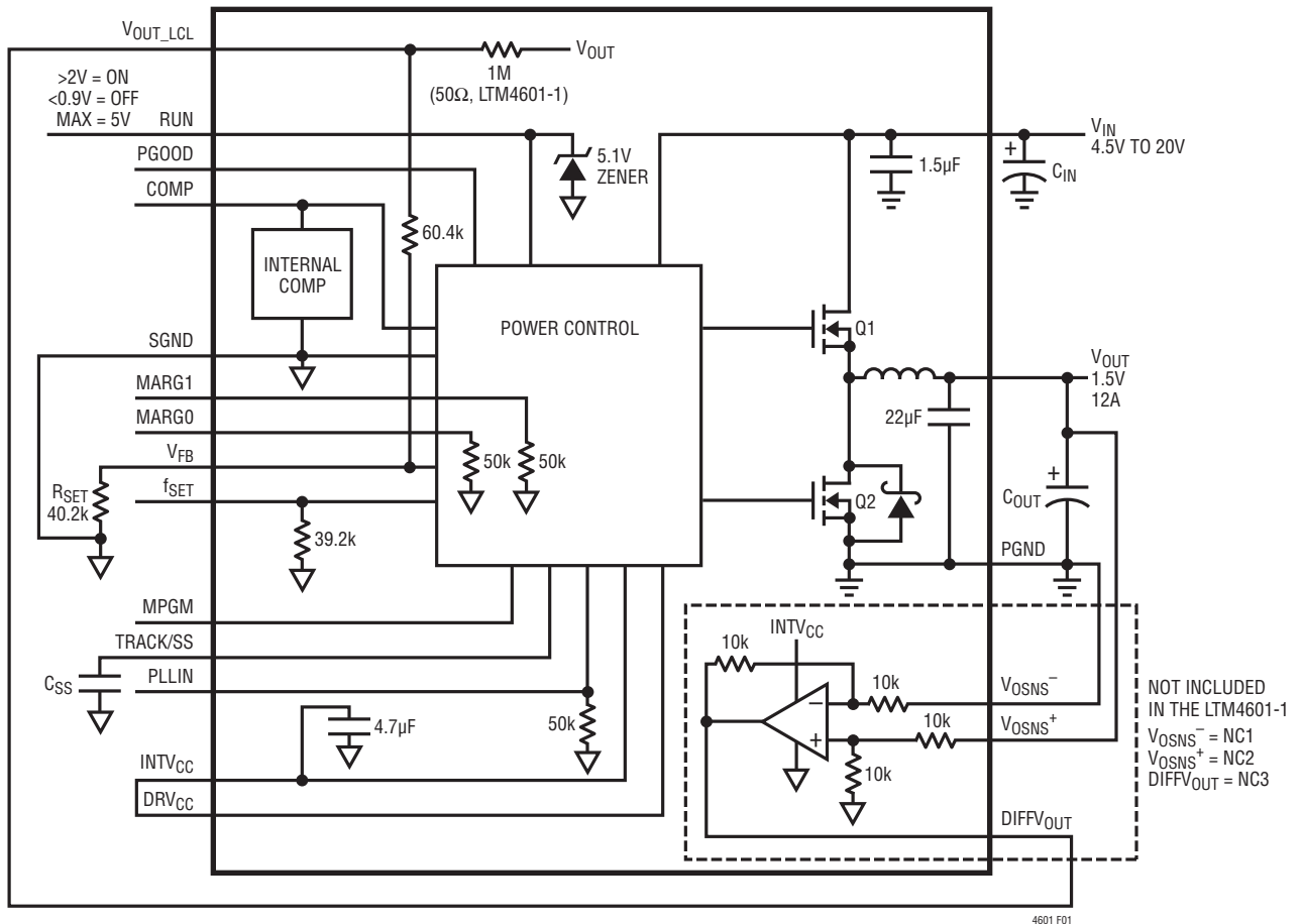
Figure 1. Simplified LTM4601/LTM4601-1 Block Diagram
