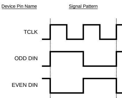
Figure 1. Serializer Input Checker-board Pattern
