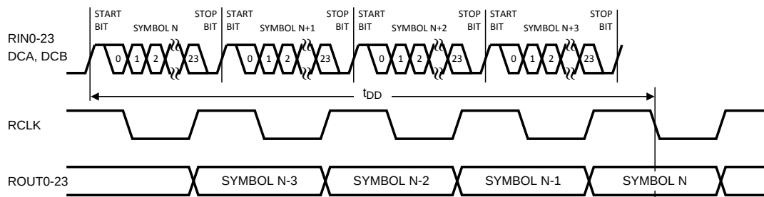
Figure 12. Deserializer Delay
