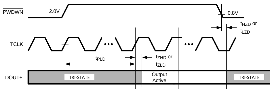
Figure 7. Serializer PLL Lock Time, and TPWDB TRI-STATE Delays
