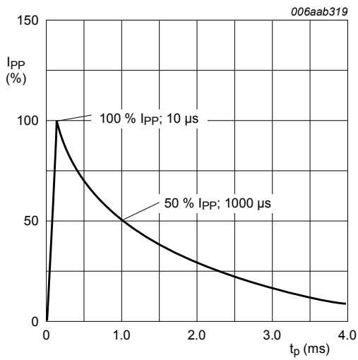
Fig. 2. 10/1000 \mu\text{s} pulse waveform according to IEC 61643-321
