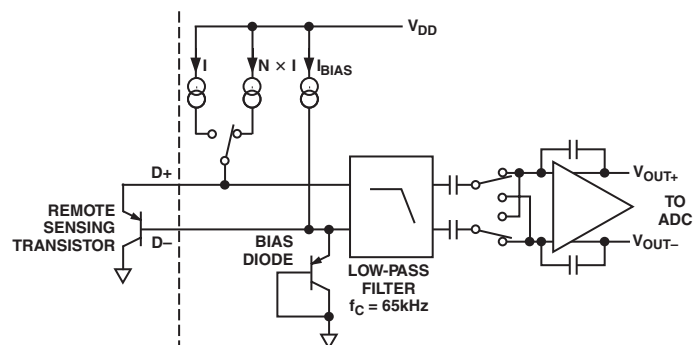
Figure 3. Signal Conditioning
