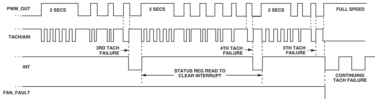
Figure 22. Operation of \text{FAN\_FAULT} and Interrupt Pins
