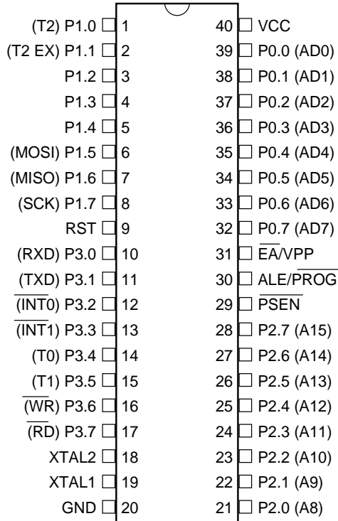
PDIP
