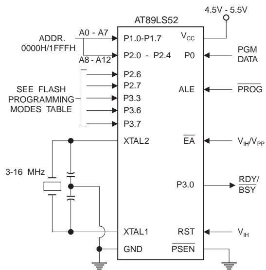
Figure 9. Programming the Flash Memory (Parallel Mode)
