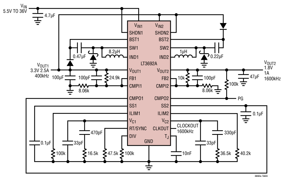
3.3V and 1.8V 2-Stage Dual Step-Down Multi-Frequency Converter
