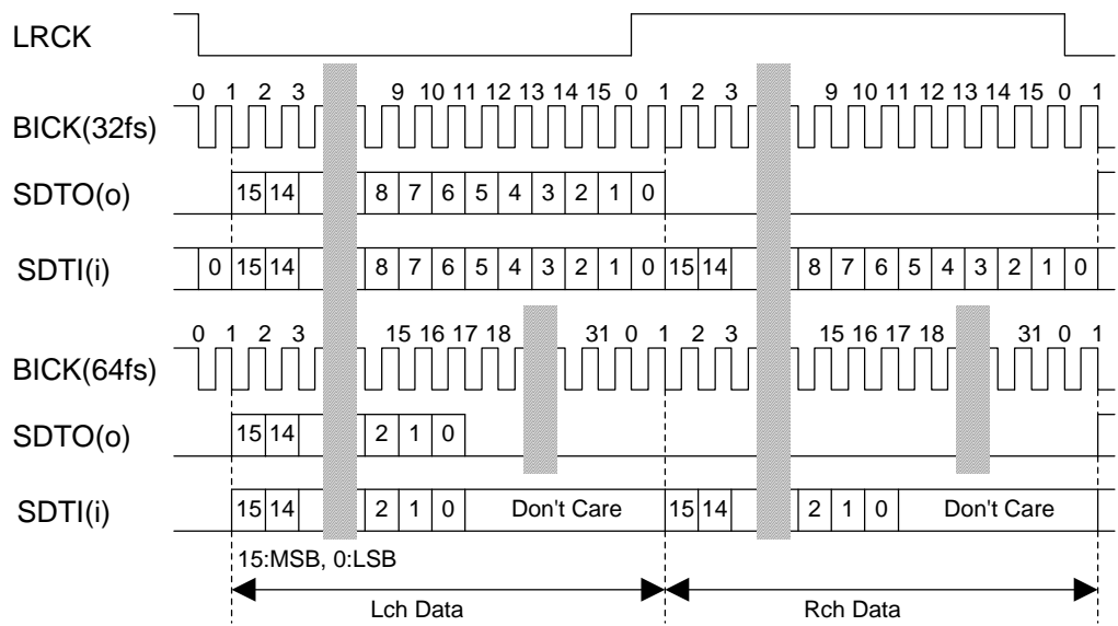
Figure 16. Mode 2 Timing
