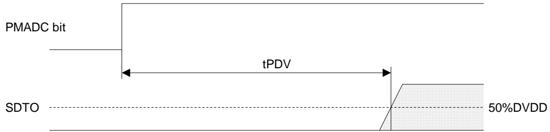
Figure 9. Power Down & Reset Timing 1
