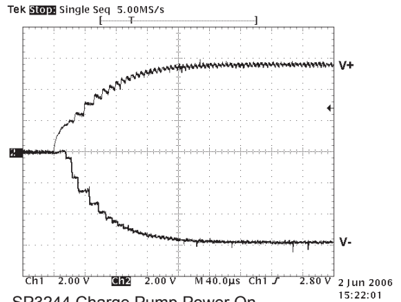
SP3244 Charge Pump Power On TimeVcc=3.3V, T=27C
