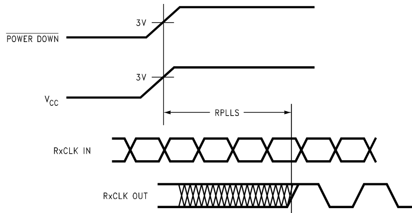
Figure 8. DS90CR218 (Receiver) Phase Lock Loop Set Time
