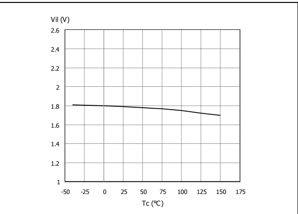
Figure 18. Input low-level
