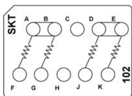
CTJ420E102 Two 20 k \Omega Resistors, 1/4 W Two 8.45 k \Omega Resistors, 1/4 W
