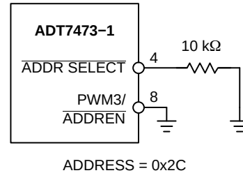
Figure 14. SMBus Address = 0x2C (Pin 4 = 0)
