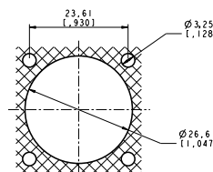
PERCAGE PANNEAU PANEL DRILLING
