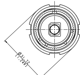
Panel Drilling
