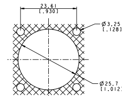
Panel Drilling
