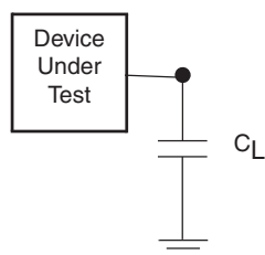
Figure 14.2 Test Setup
