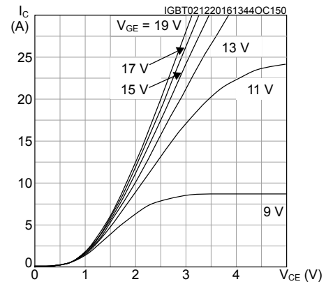
Figure 6. IGBT output characteristics ( T_J = 150\text{ °C} , terminal)
