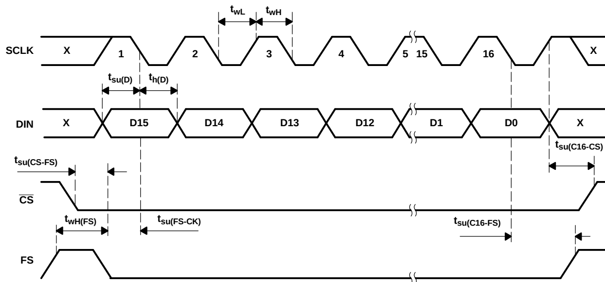
Figure 1. Timing Diagram
