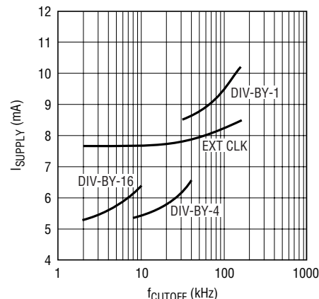
3V Supply Current
