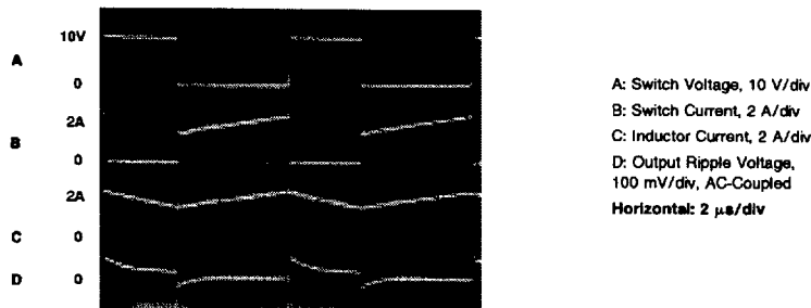
FIGURE 31. Switching Waveforms
