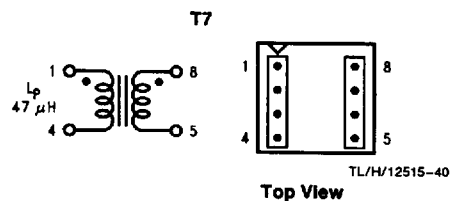
FIGURE 24. Renco RL-5751
