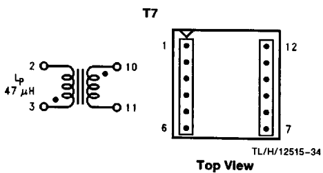
FIGURE 19. Collcraft S6057-A (Surface Mount)
