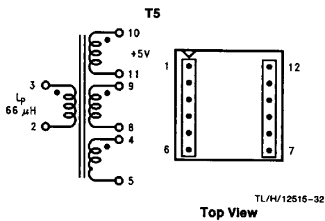
FIGURE 17. Collcraft Q4437-B (Surface Mount)
