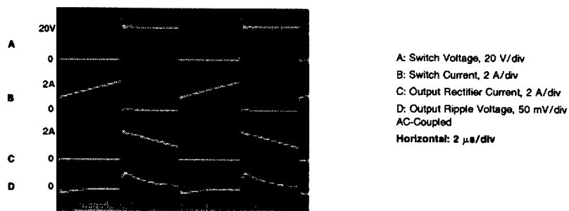
FIGURE 5. Switching Waveforms
