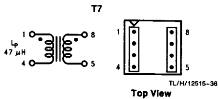
FIGURE 21. Pulse PE-68482
