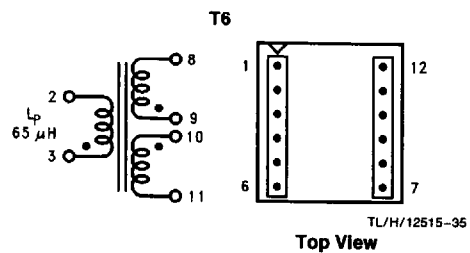
FIGURE 20. Collcraft Q4438-B (Surface Mount)
