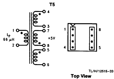
FIGURE 18. Collcraft Q4338-B
