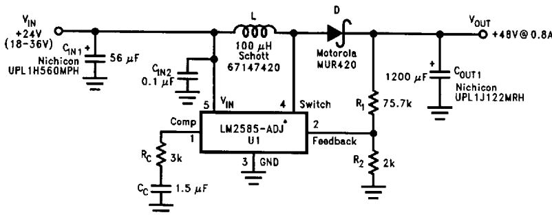
FIGURE 37. +24V to +48V Boost Regulator
