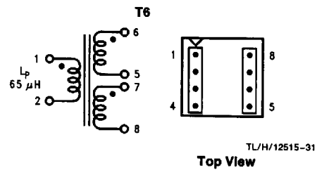
FIGURE 16. Collcraft Q4339-B
