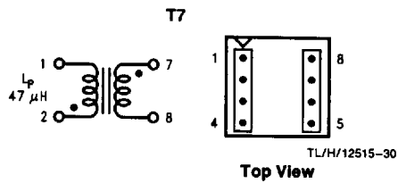
FIGURE 15. Collcraft S6000-A
