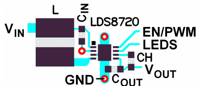
Figure 3. Recommended layout
