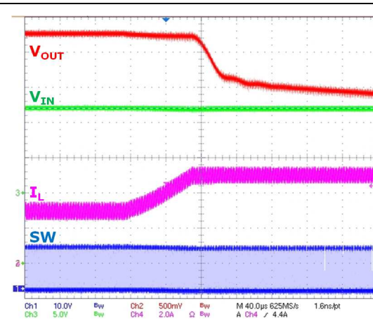
Figure 16. Overcurrent protection
