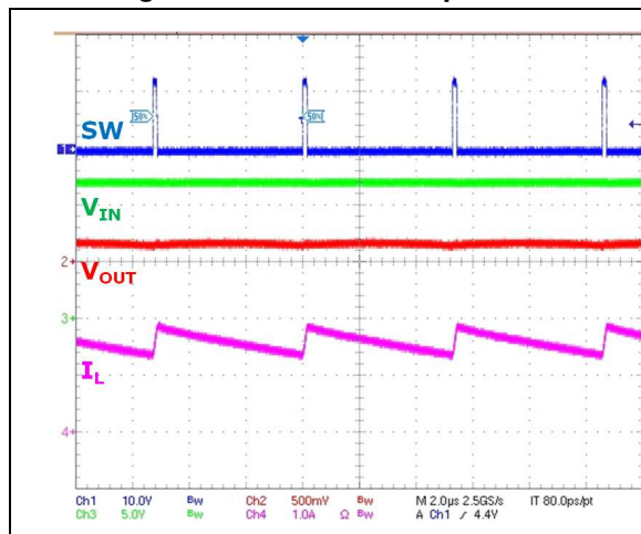
Figure 17. Short-circuit protection
