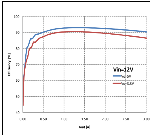
Figure 15. Efficiency vs. I_{OUT}
