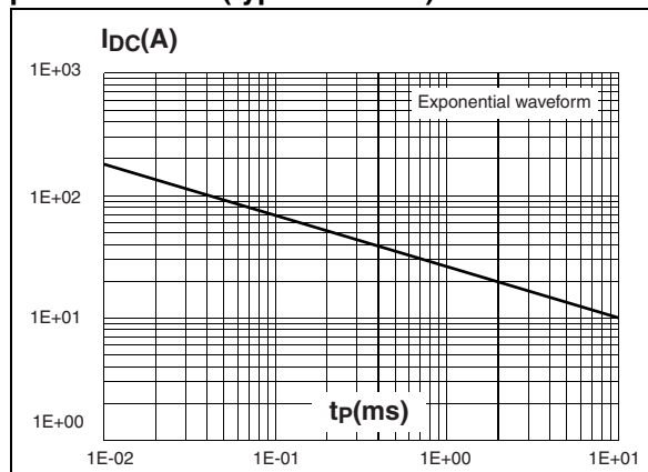
Figure 5: Peak current I_{DC} inducing open circuit of the wire for one input/output versus pulse duration (typical values)
