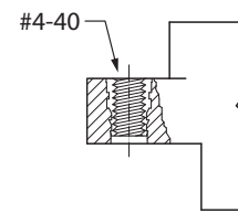
THREADED INSERT (I)
