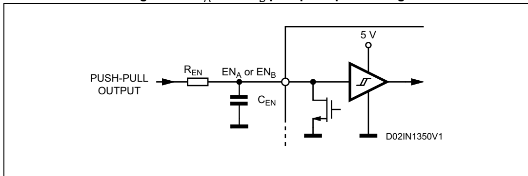
Figure 8. EN_A and EN_B pins push-pull driving
