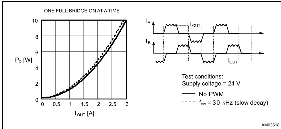
Figure 19. IC Power dissipation versus output current with one full bridge ON at a time
