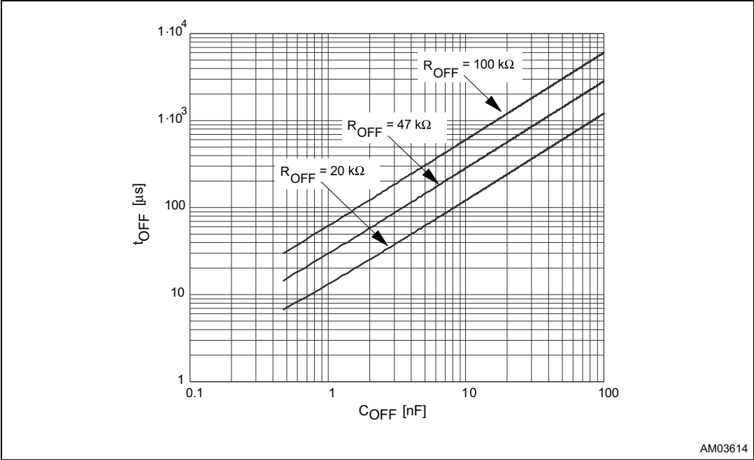
Figure 11. t_{OFF} versus C_{OFF} and R_{OFF}
