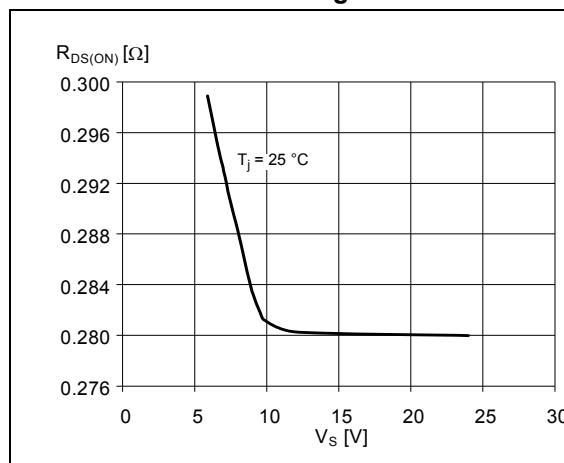
Figure 29. Typical low-side R_{DS(ON)} vs. supply voltage
