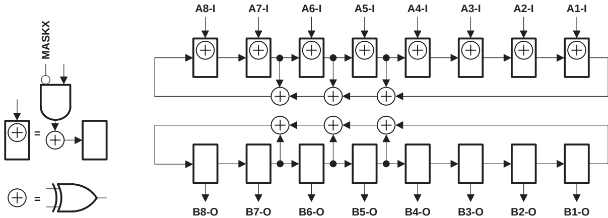
Figure 9. 8-Bit PSA/PRPG Configuration (OEA = 0, OEB = 1)
