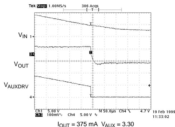
Figure 15. Power-Down, V_{AUX} = 3.3 V. Again, Note \Delta V = I R_{DS(ON)} \approx 130 mV
