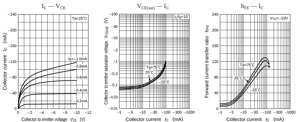
Characteristics charts of UN911L
