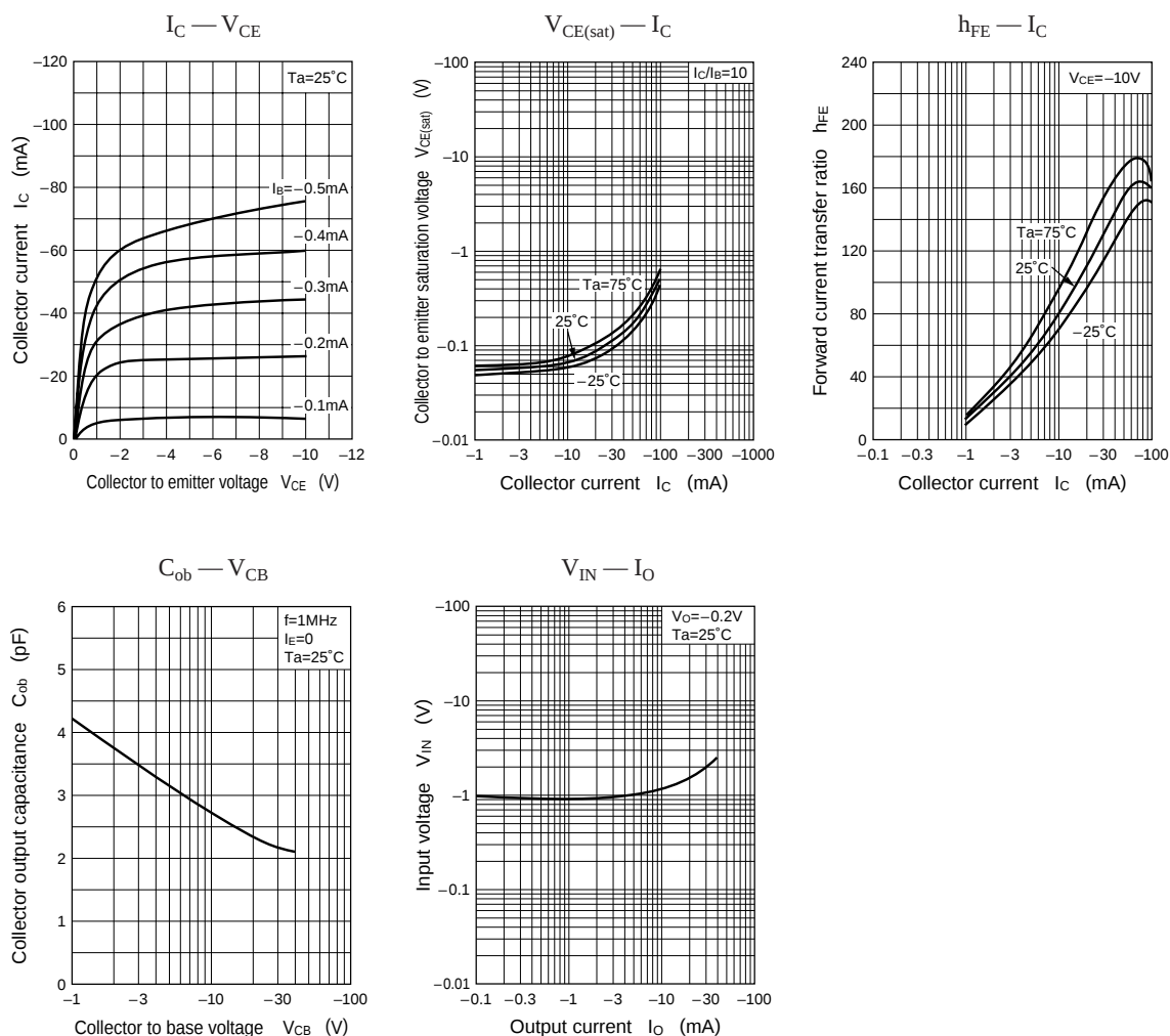
Characteristics charts of UN911L
