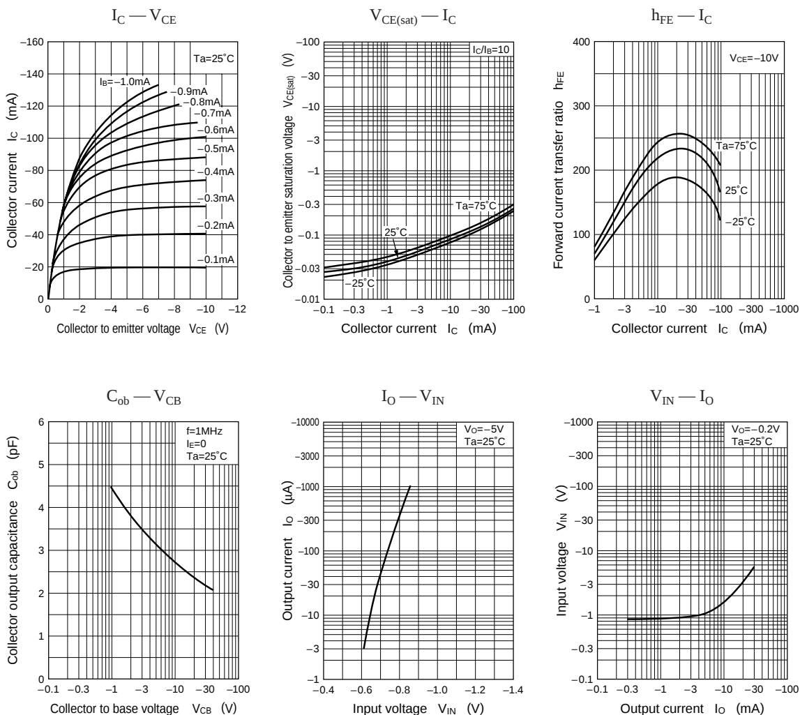
Characteristics charts of UN9114
