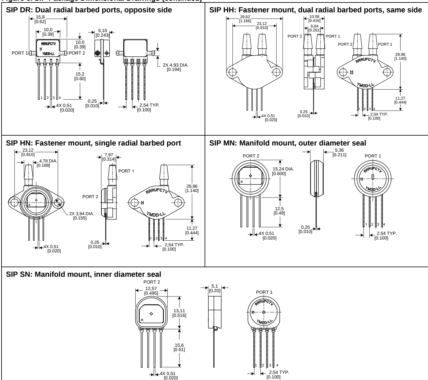
Figure 6. SIP Package Dimensional Drawings (continued)
