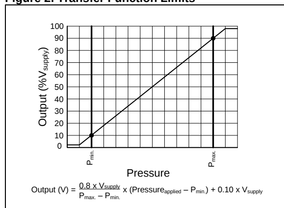
Figure 2. Transfer Function Limits
