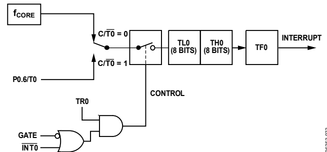
Figure 98. Timer/Counter 0, Mode 1
