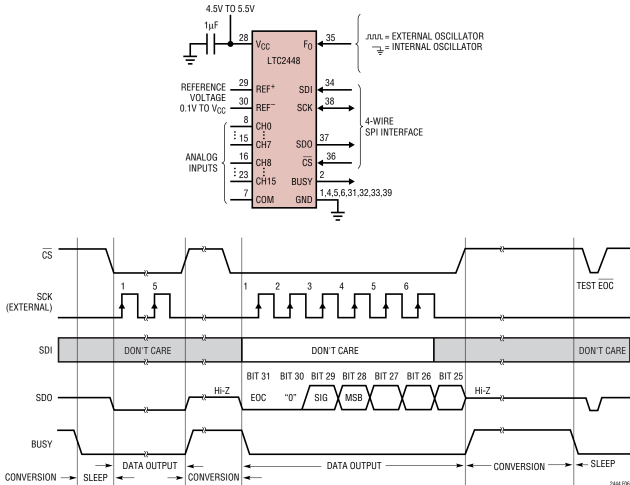
Figure 5. External Serial Clock, Reduced Output Data Length
