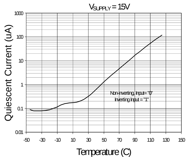
Fig. 15 Quiescent Current vs. Temperature V_{\text{SUPPLY}} = 15\text{V}
