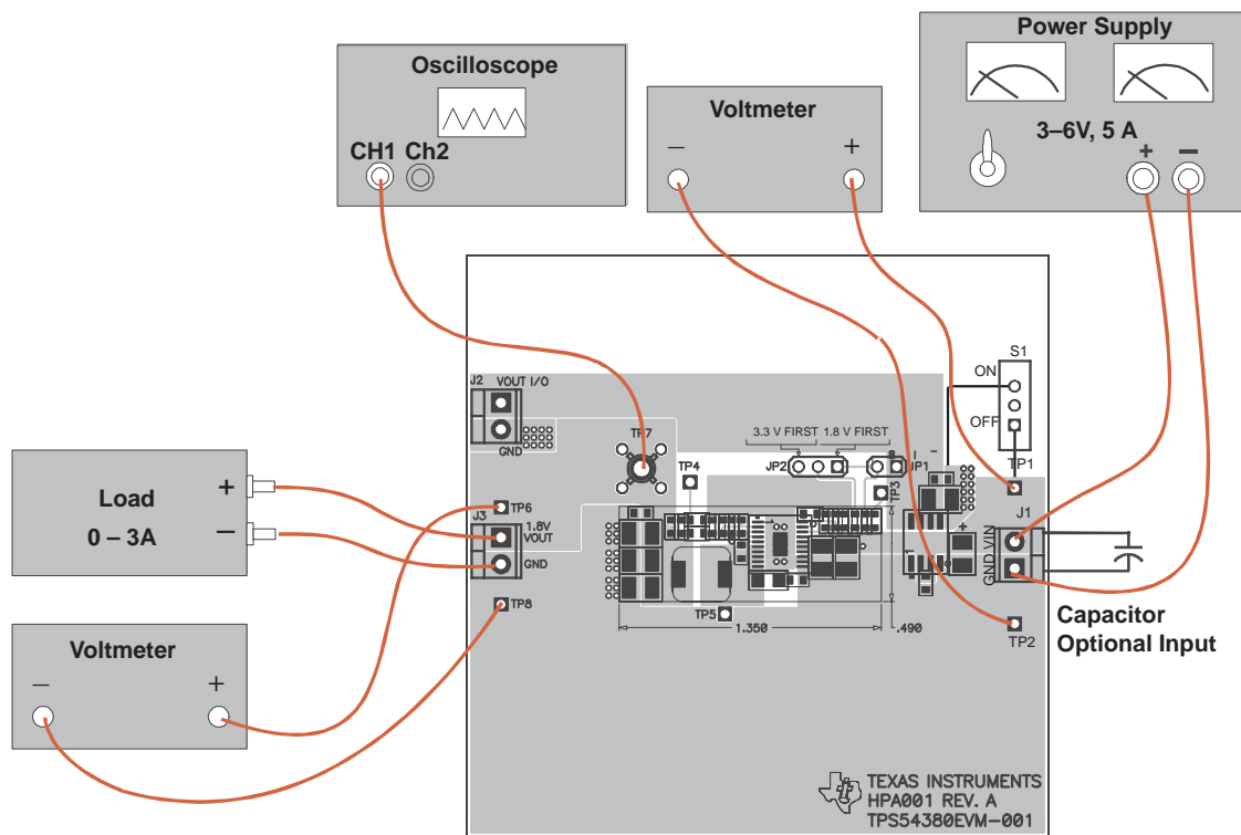
Figure 2–1. Connection Diagram
