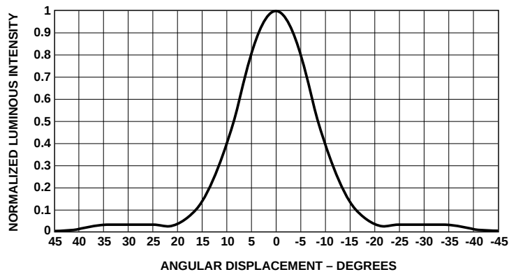
Figure 6. Relative Luminous Intensity vs. Angular Displacement. 15 Degree Family.
