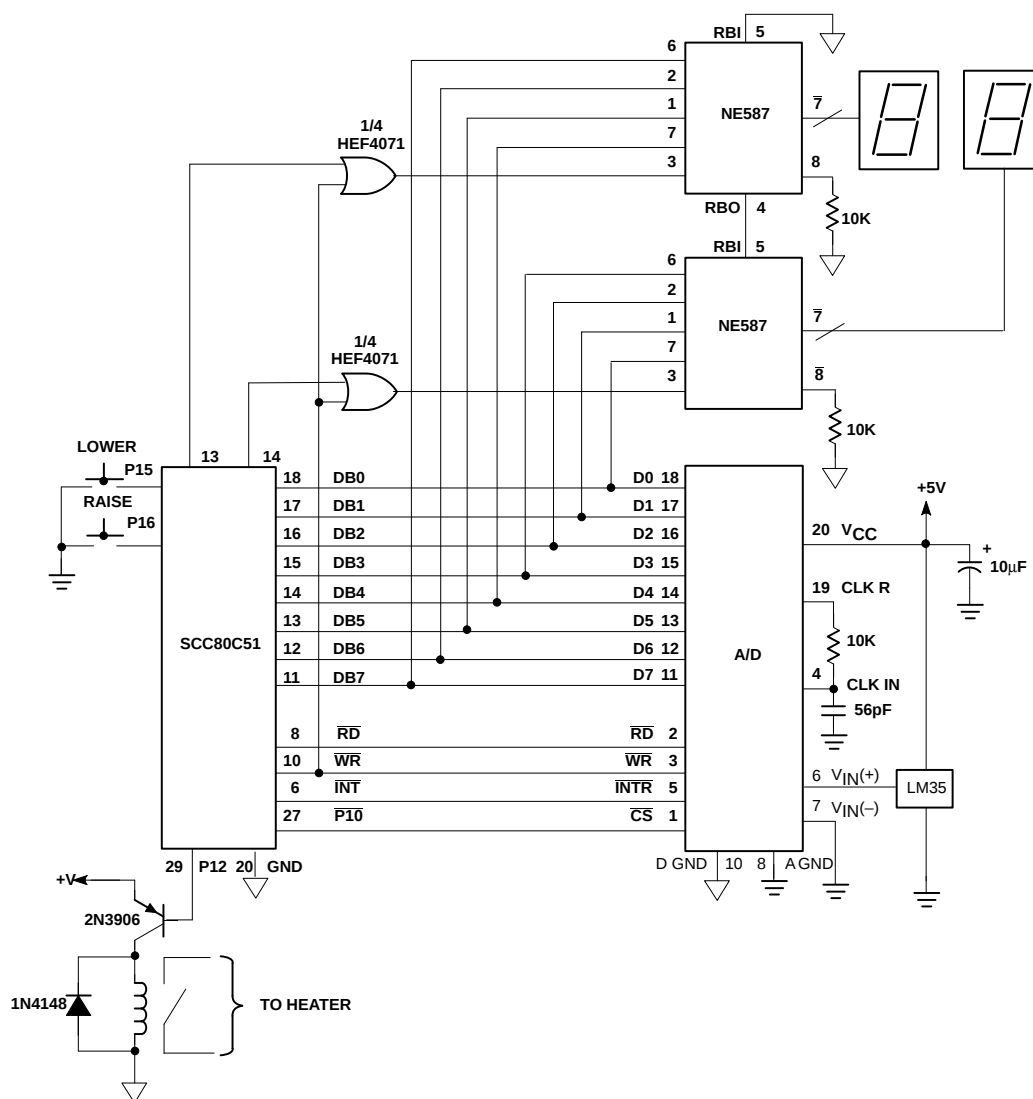
Figure 11. Digital Thermostat
