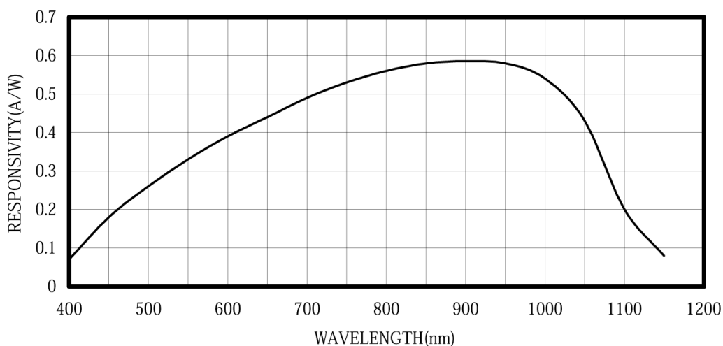
RESPONSIVITY
