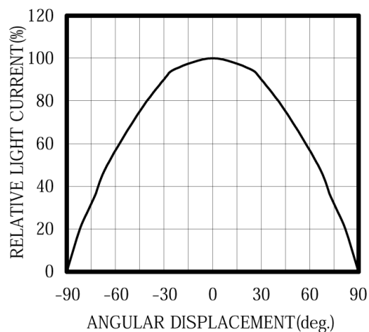
ANGULAR DISPLACEMENT
