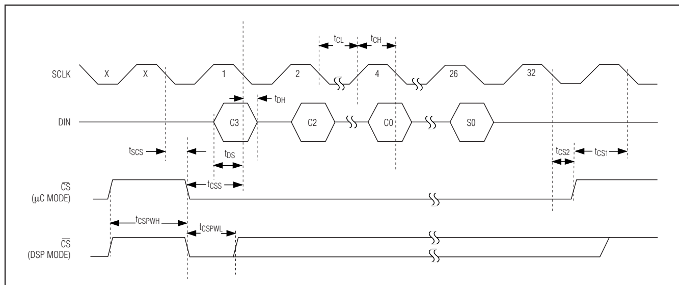
Figure 1. Serial-Interface Timing
