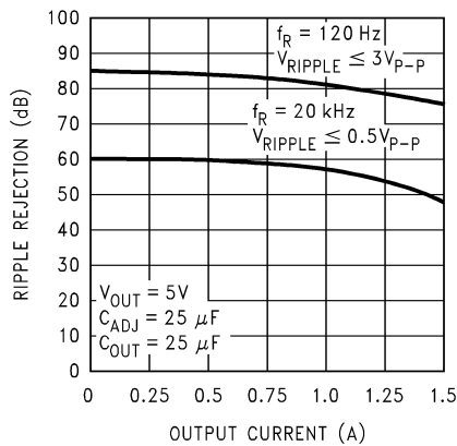
LM1084-ADJ Ripple Rejection vs Current
