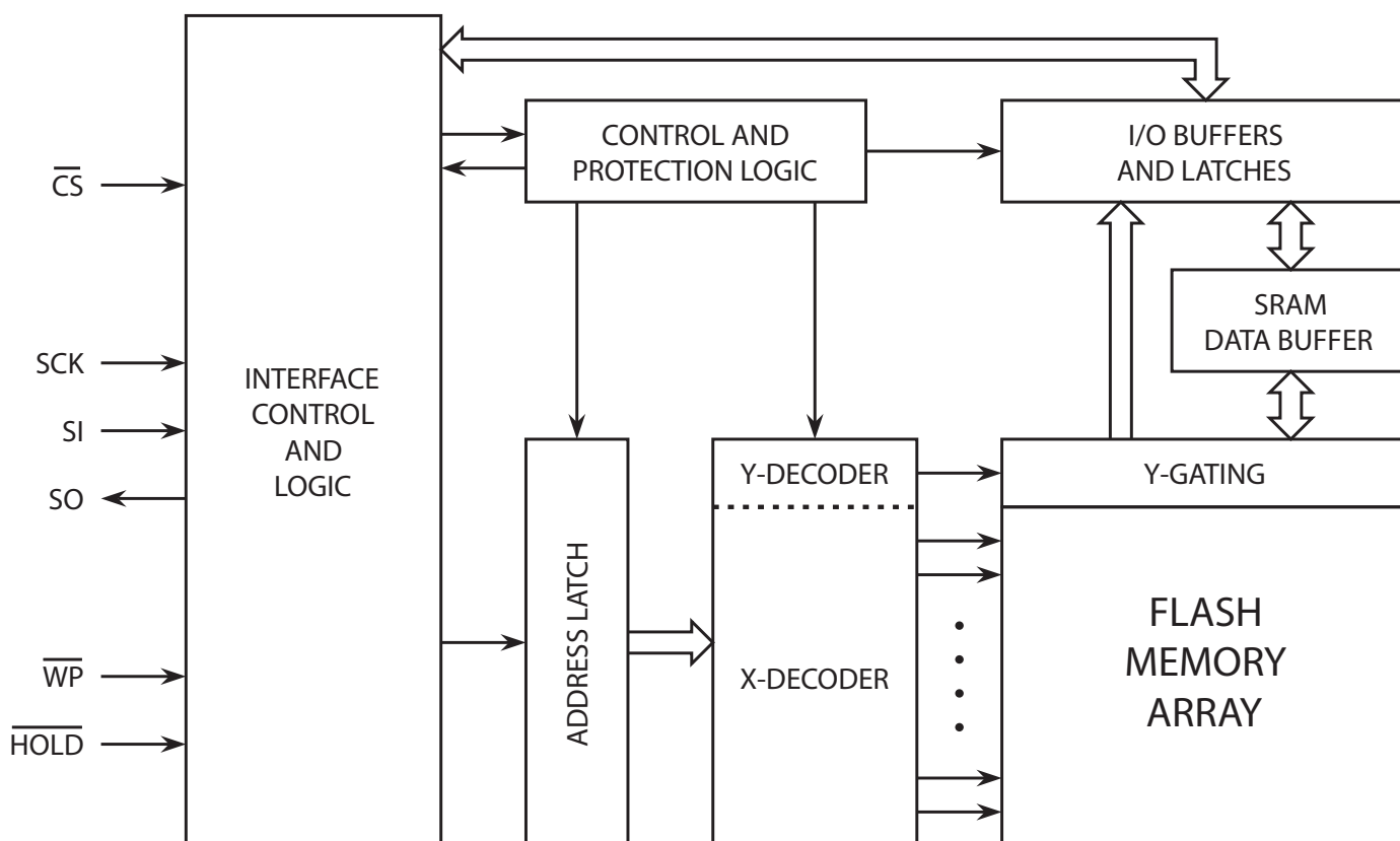
Figure 3-1. Block Diagram
