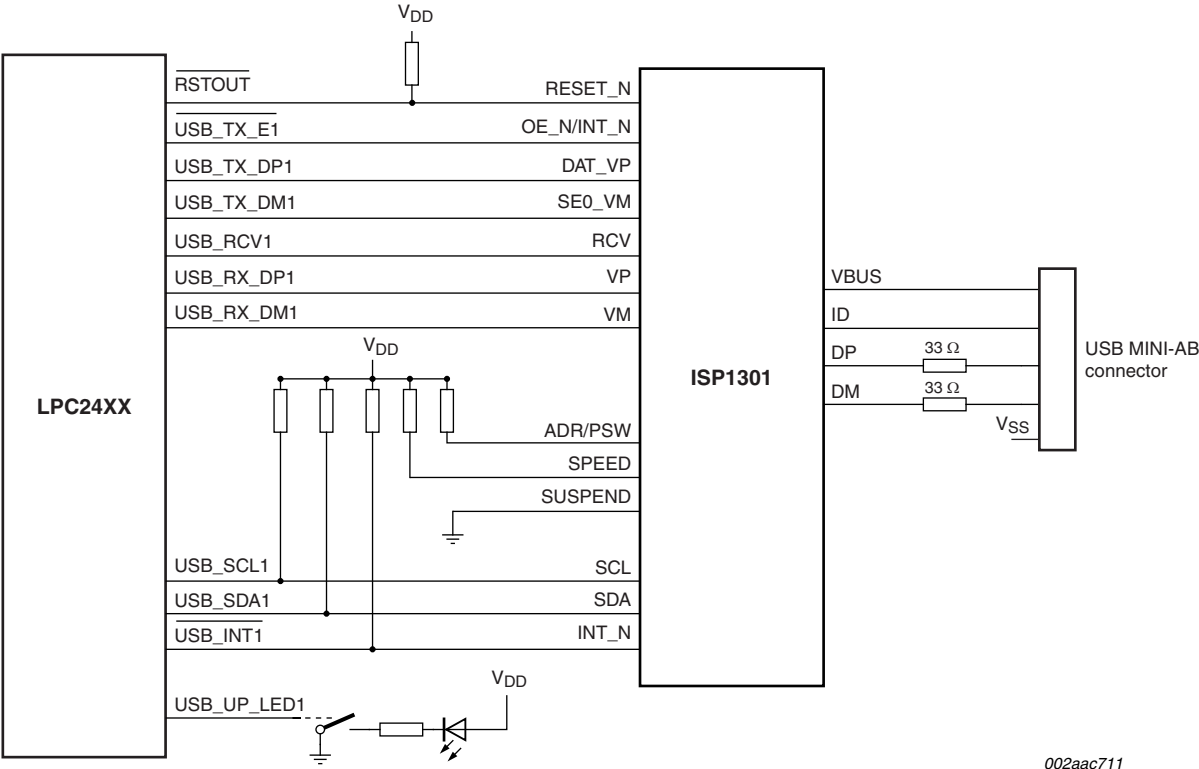
Fig 14. LPC2478 USB OTG port configuration: VP_VM mode
