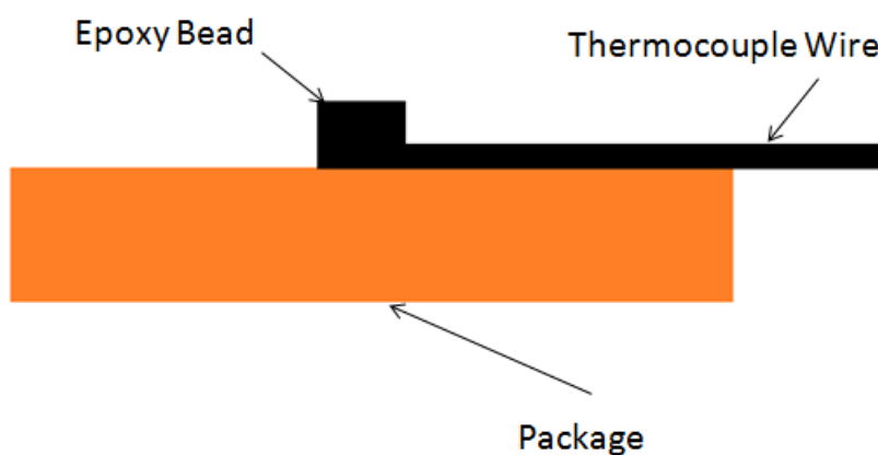
Figure 12-18. Technique for Measuring T_{\text{case}} with 0° Angle Attachment, No Heat Sink
