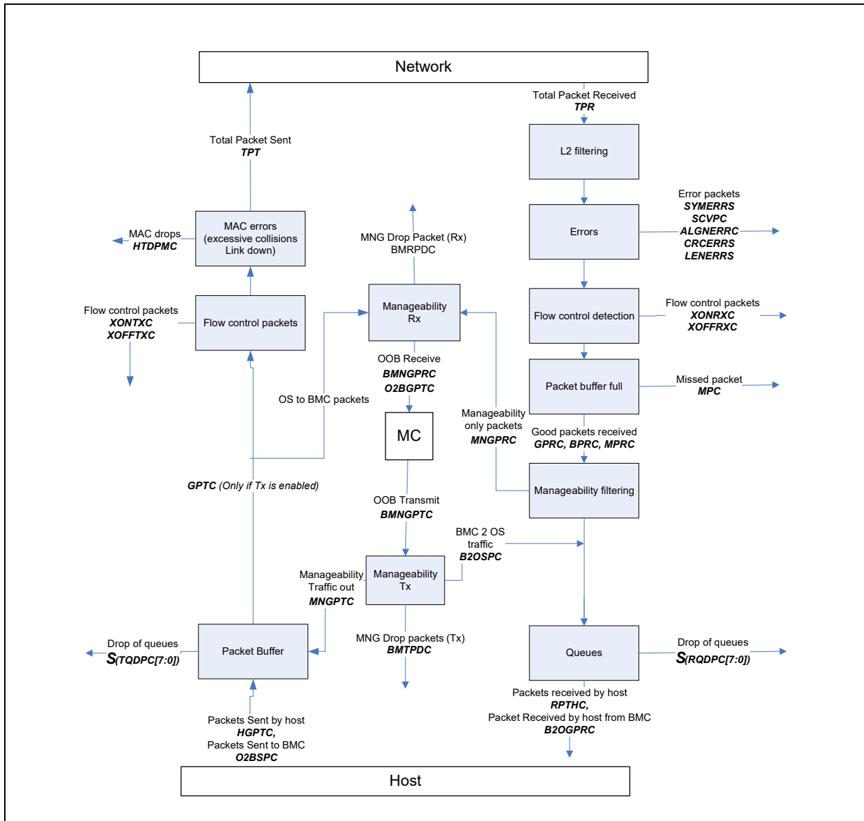
Figure 7-17. Flow Statistics
