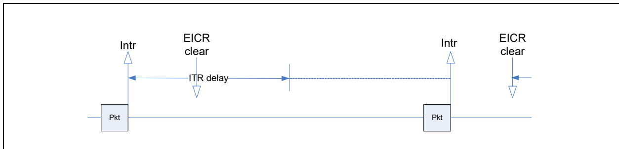
Figure 7-12. Light load, Interrupts Immediately on Packet Receive
