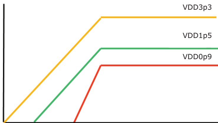
Figure 11-12. Power Sequencing Guideline
