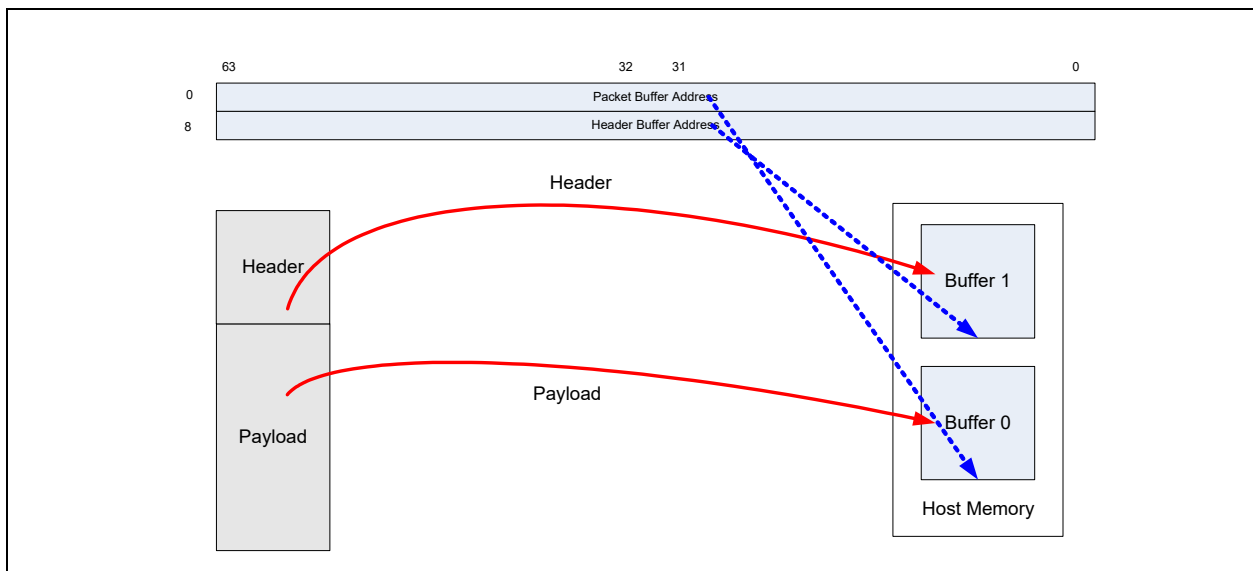
Figure 7-5. Header Splitting
