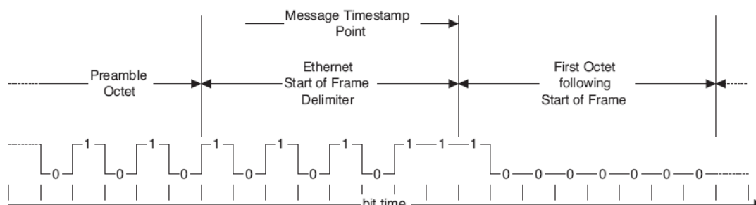
Figure 7-16. Timestamp Point
