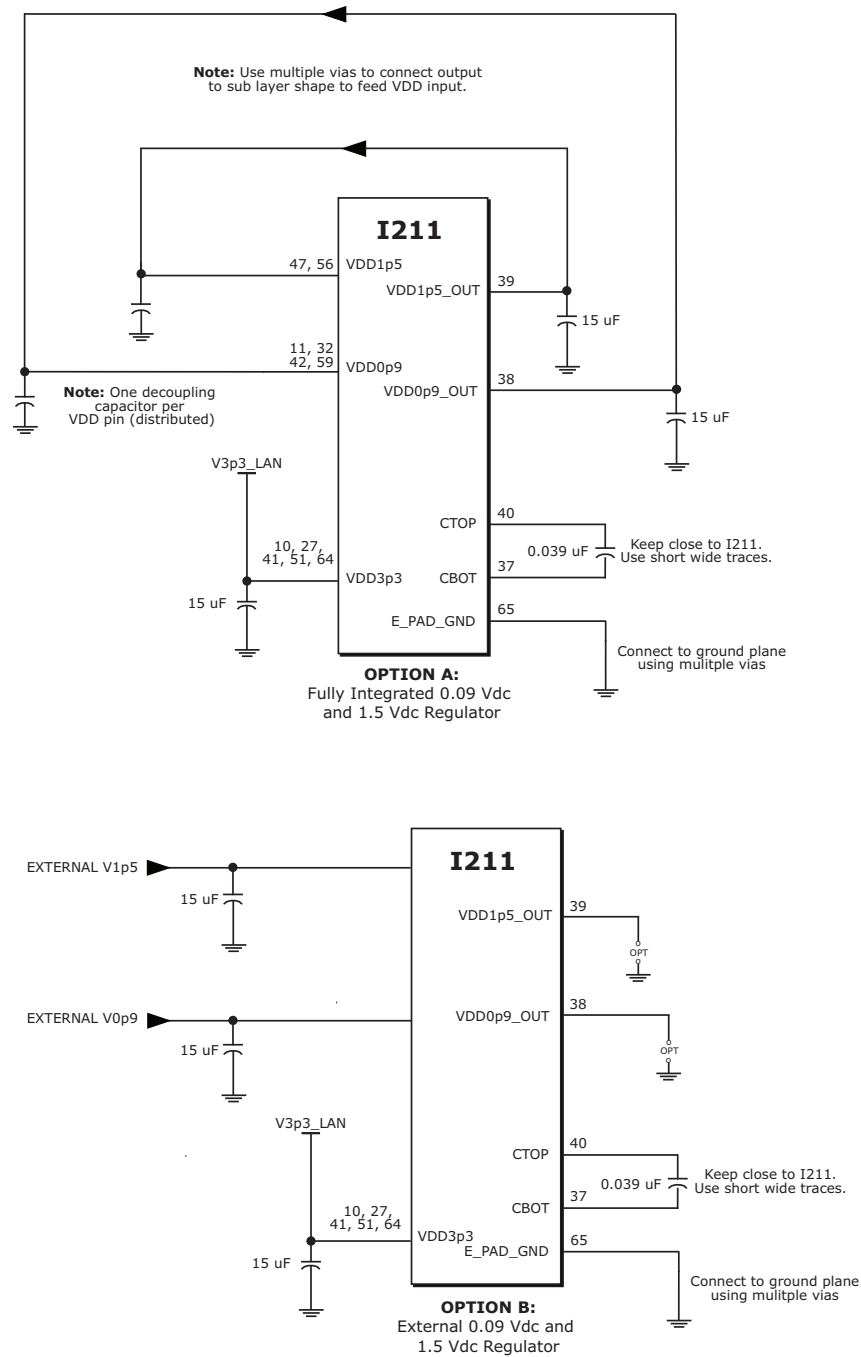
Figure 11-11. Power Delivery Solutions
