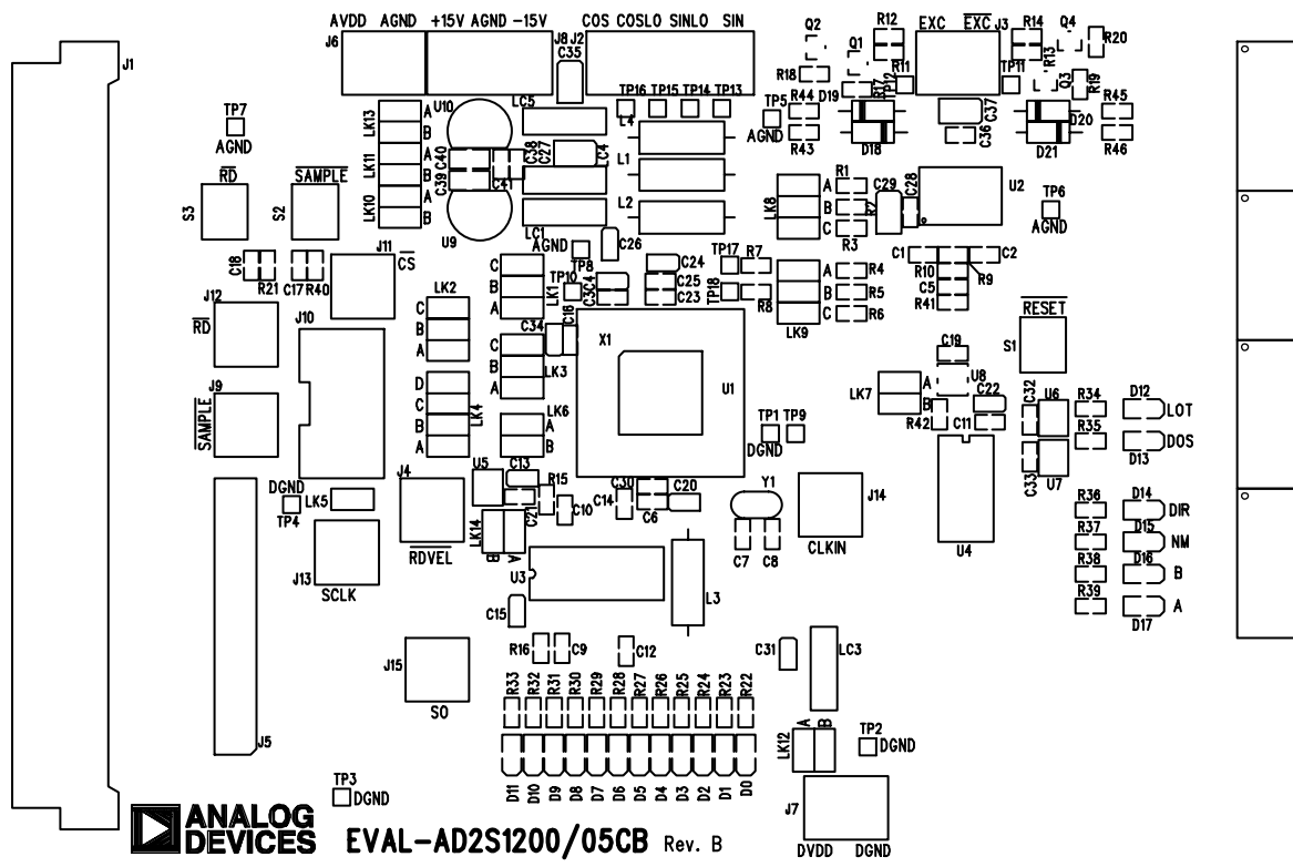
Figure 8. Silkscreen Image
