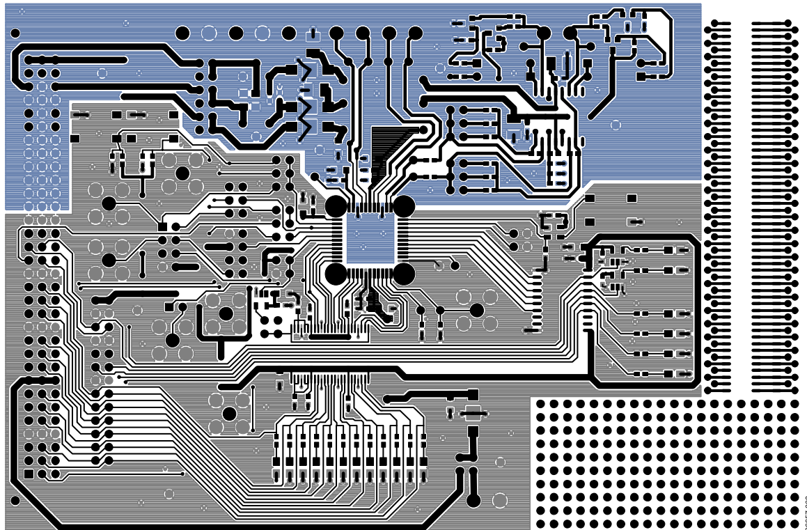
Figure 9. Component Side
