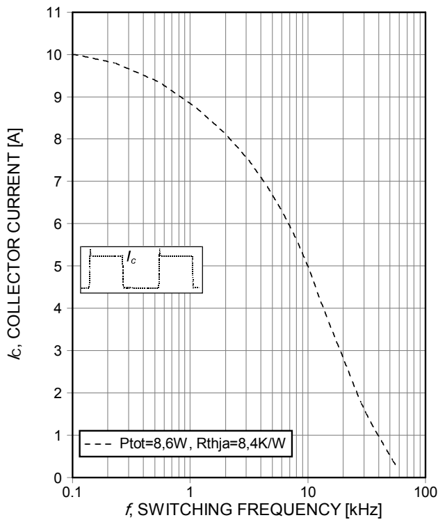
Figure 1. Collector current as a function of switching frequency (T_{vj} \leq 175^\circ C, T_a = 55^\circ C, D = 0.5, V_{CE} = 400V, V_{GE} = 15/0V, r_G = 23\Omega, \text{PCB mounting with thermal vias and heatsink, see Appnote: } \text{www.infineon.com/igbt})
