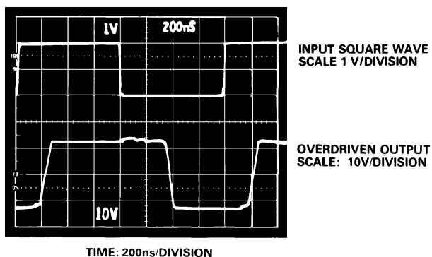
Figure 26. Overdrive Recovery
