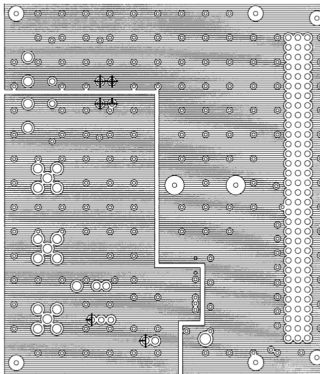
FIGURE 3. POWER LAYER (2)
