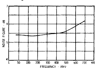
Noise Figure
