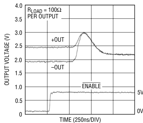
Turn-Off Time
