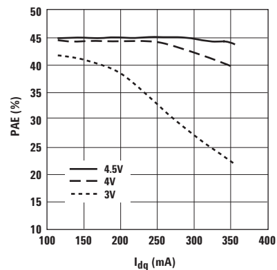
Figure 19. PAE @ P1dB vs. I_{dq} and V_{ds} at 3.9 GHz.
